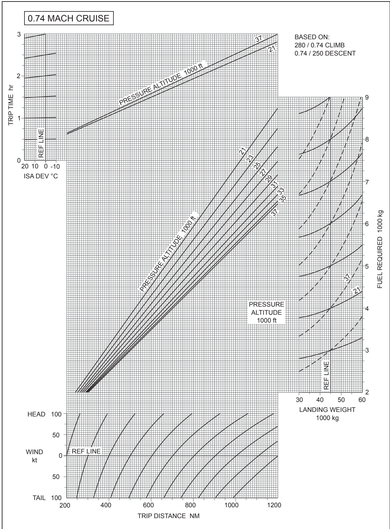
Figure 4.3.2b Simplified Flight Planning – Trip Distances 200 NM to 1,200 NM
